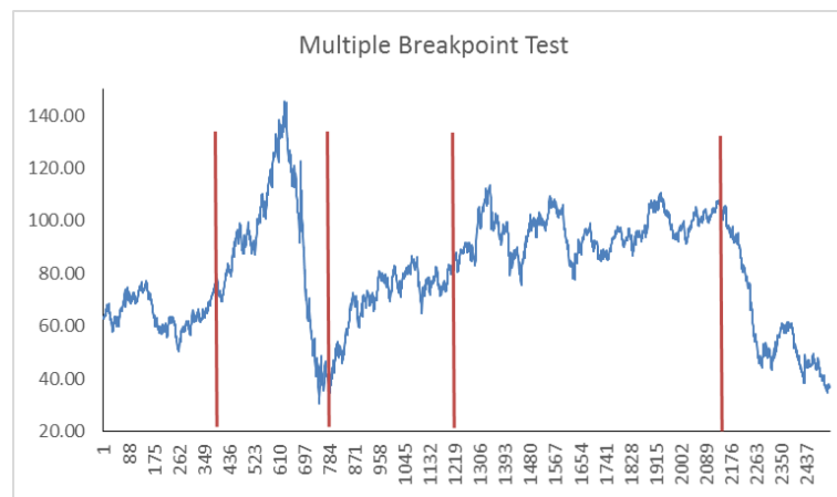
Figure no. 4 – The plot of multiple-breakpoint tests for daily WTI crude oil prices between 3 January, 2006 and 31 December, 2015
