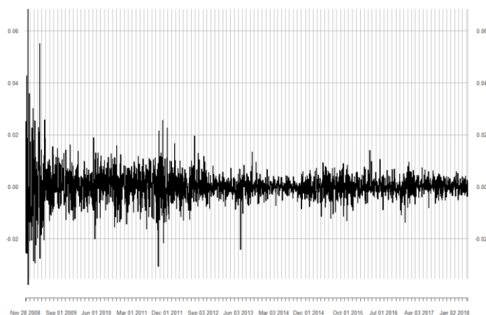
Figure no. 2 – Daily changes of S&P Green Bond index values (period 2008-11-28 to 2018-04-13)
