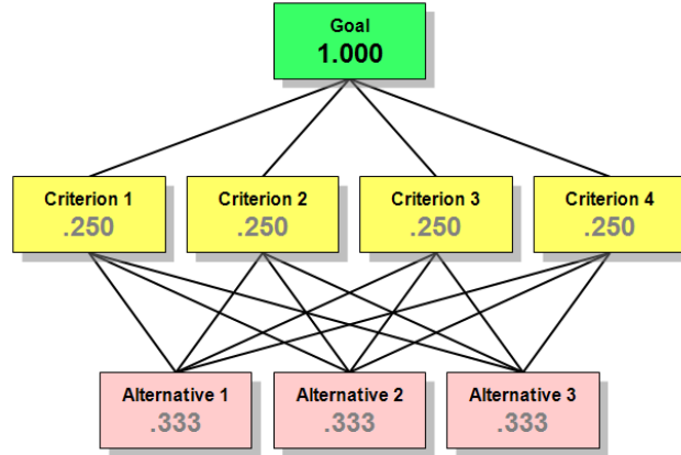
Figure no. 1 – Three-level hierarchical structure of DM problem with 4 criteria and 3 alternatives
