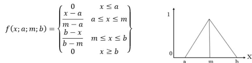
Figure no. 7 – The shape of triangular membership function
