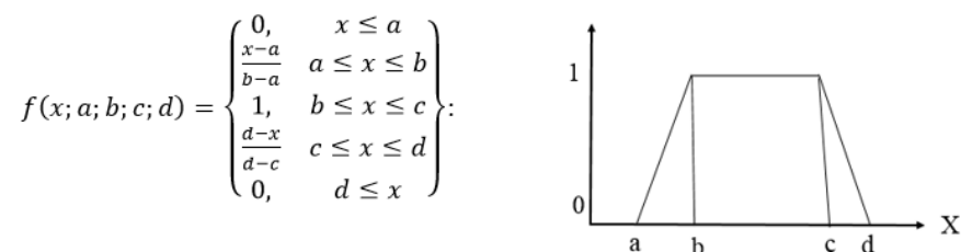
Figure no. 6 – The shape of trapezoidal membership function
